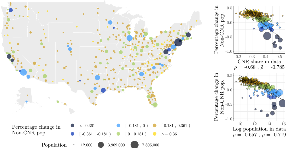
Figure 10: L_n^{CNR} (percentage change from data equilibrium)
